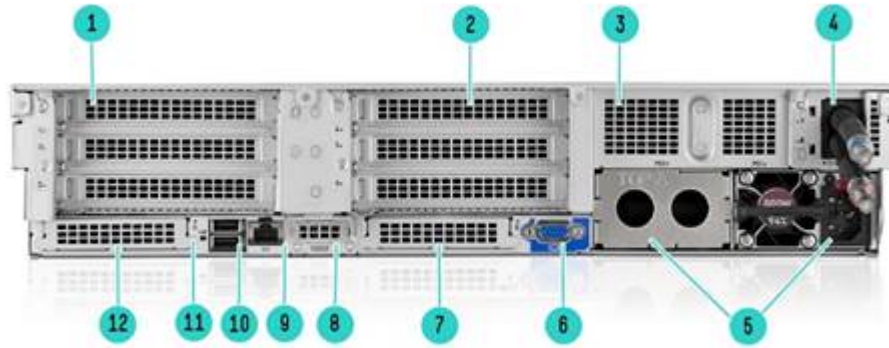
Rear View - DL380 Gen12 Direct Liquid Cooling
